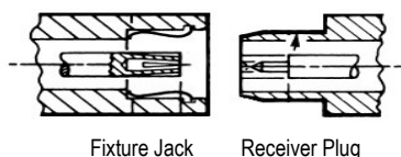
Fixture Jack
